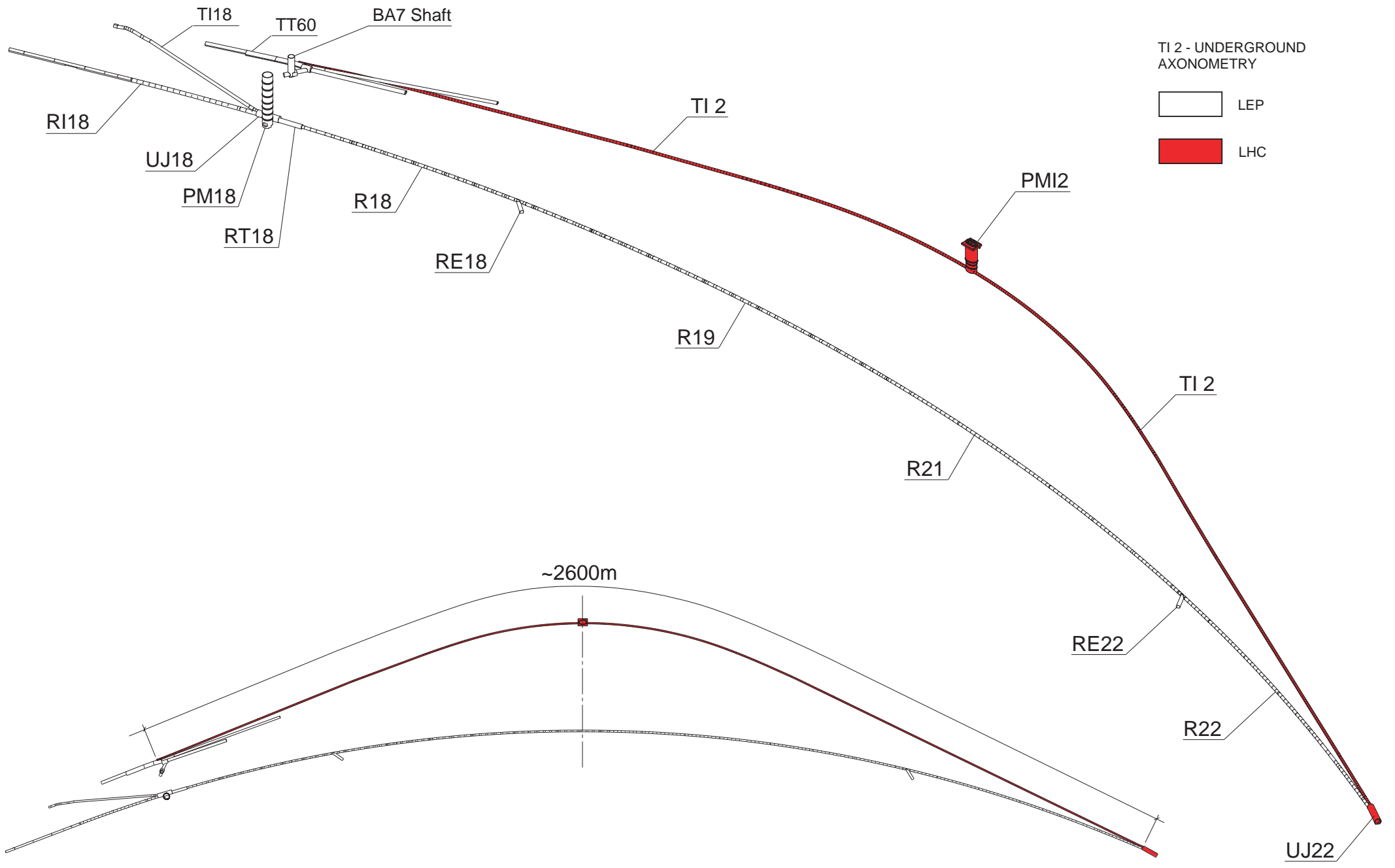
TI 2 - UNDERGROUND LAYOUT
