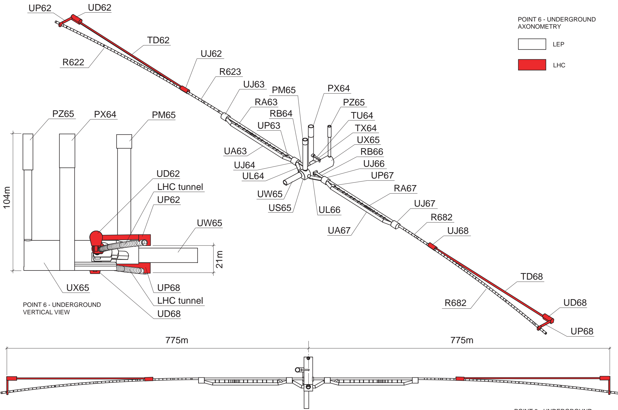
POINT 6 - UNDERGROUND LAYOUT
